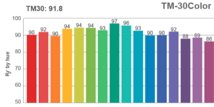
Color distortion
